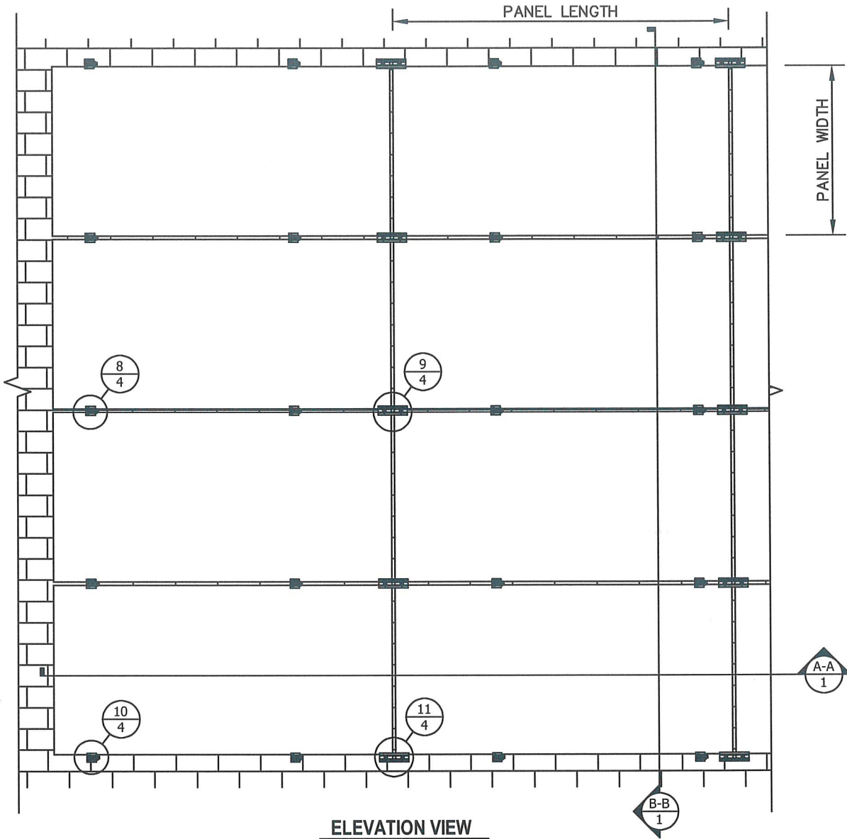
ELEVATION VIEW
